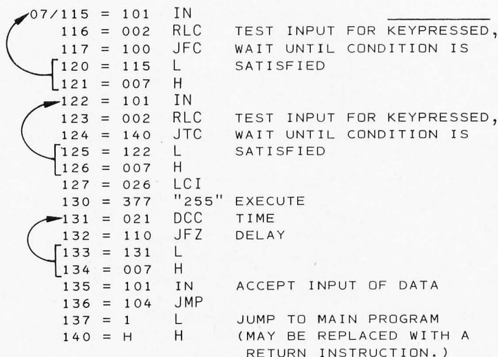
Fig. 3. Software can be used to debounce a keyboard — simply loop around for a long enough time to ensure that keys have stabilized. The loop is started as soon as the "any key pressed" ( keypressed ) line indicates any non-null bit pattern.
